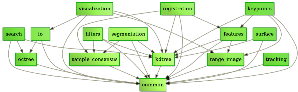
Fig. 11. PCL dependency graph.
