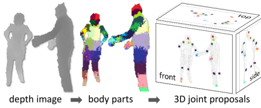
Fig. 17. Human Pose Recognition.
