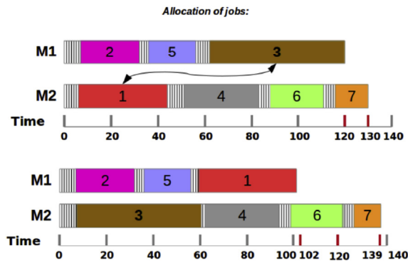
(c) Swap between different machines
