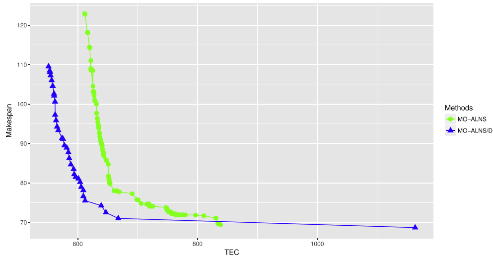
Fig. 13. Pareto front obtained with the MO-ALNS and MO-ALNS/D algorithms for an instance with 50 jobs and 10 machines.
