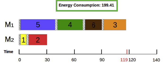
Fig. 2. Optimal solution for the minimization of the total energy consumption.
