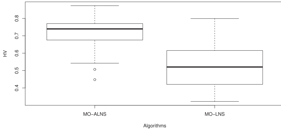
Fig. 8. Box plot results of the MO-ALNS and MO-LNS algorithms for the HV indicator.
