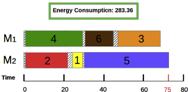
Fig. 1. Optimal solution for the minimization of the makespan .
