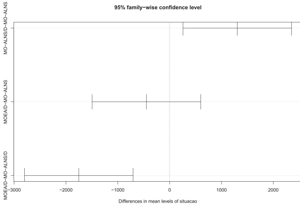
Fig. 12. Tukey HSD test results for the HCC indicator.
