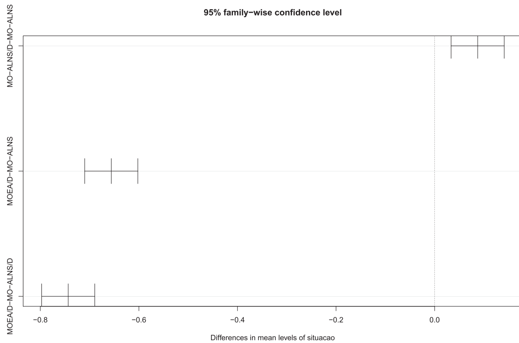
Fig. 11. Tukey HSD test results for the HV indicator.
