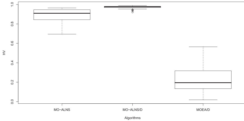
Fig. 9. Box plot results of the MO-ALNS, MO-ALNS/D and MOEA/D algorithms for the HV indicator.
