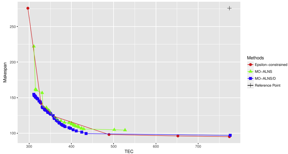
Fig. 7. Pareto front obtained with the two algorithms proposed and the \epsilon -constrained method for an instance with 12 jobs and 4 machines.
