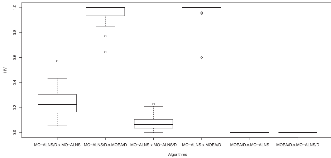
Fig. 10. Box plot results of the MO-ALNS, MO-ALNS/D and MOEA/D algorithms for the CS indicator.
