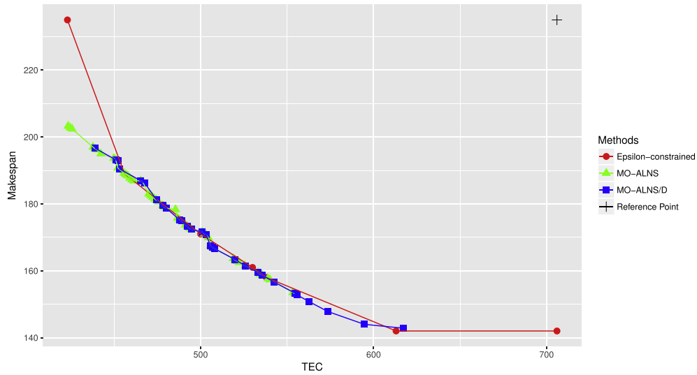
Fig. 6. Pareto front obtained with the two algorithms proposed and the \epsilon -constrained method for an instance with 8 jobs and 2 machines.
