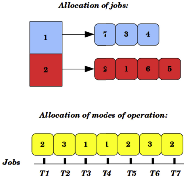
Fig. 3. Solution representation.
