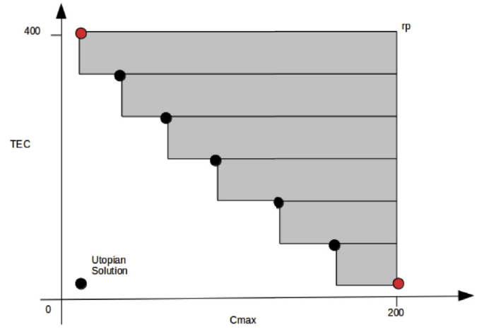
Fig. 5. Example of the hypervolume indicator.
