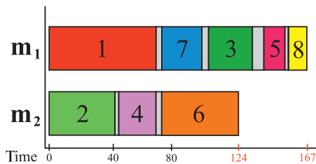
Fig. 8. A UPMSPT-ST solution.
