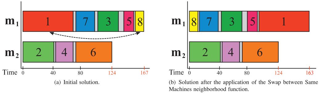
Fig. 12. Example: Swap between Same Machines neighborhood.
