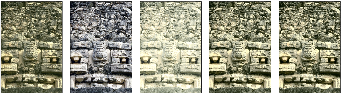
Figure 274: Results for the "33039.png" image: (a) original image; (b) C1DHE ; (c) TV3DHE ; (d) our HP1DHE ; (e) our HP2DHE .
