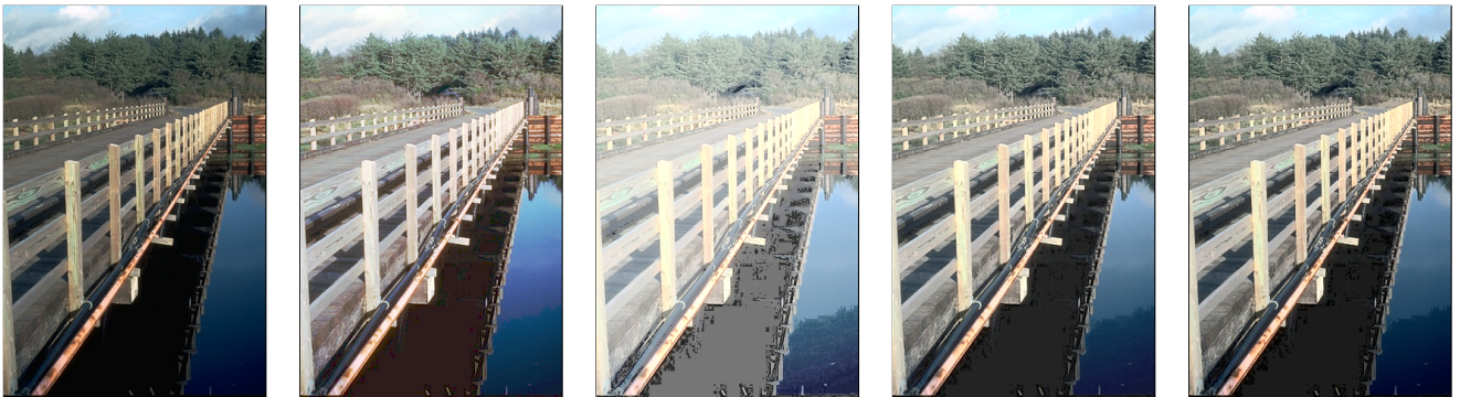
Figure 198: Results for the "22013.png" image: (a) original image; (b) C1DHE ; (c) TV3DHE ; (d) our HP1DHE ; (e) our HP2DHE .
