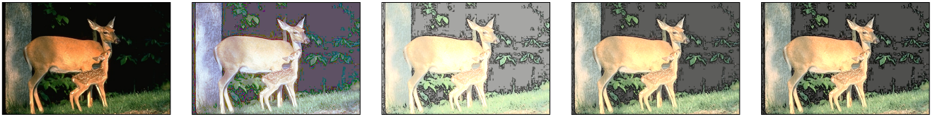
Figure 83: Results for the "317080.png" image: (a) original image; (b) C1DHE; (c) TV3DHE; (d) our HP1DHE; (e) our HP2DHE.
